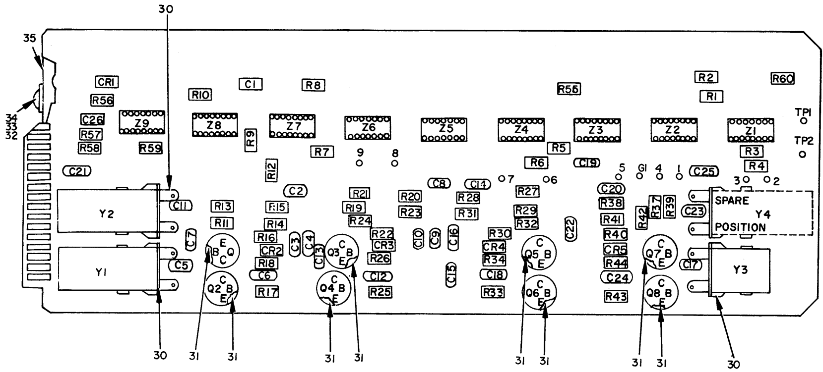
Figure 14. Component Board Assembly SMD633061 1A2A11 (Sheet 1 of 2).
