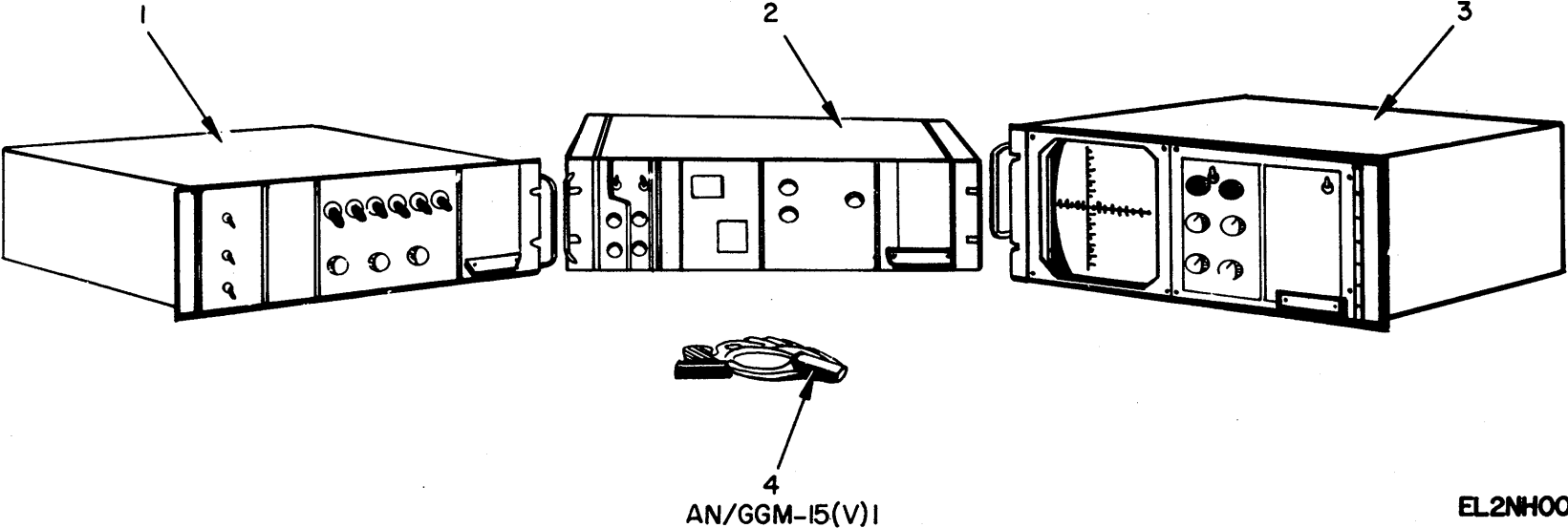
Figure 1. Test Sets, Telegraph AN/GGM-15(V)1 and AN/GGM-15(V)2 (Sheet 1 of 2).
