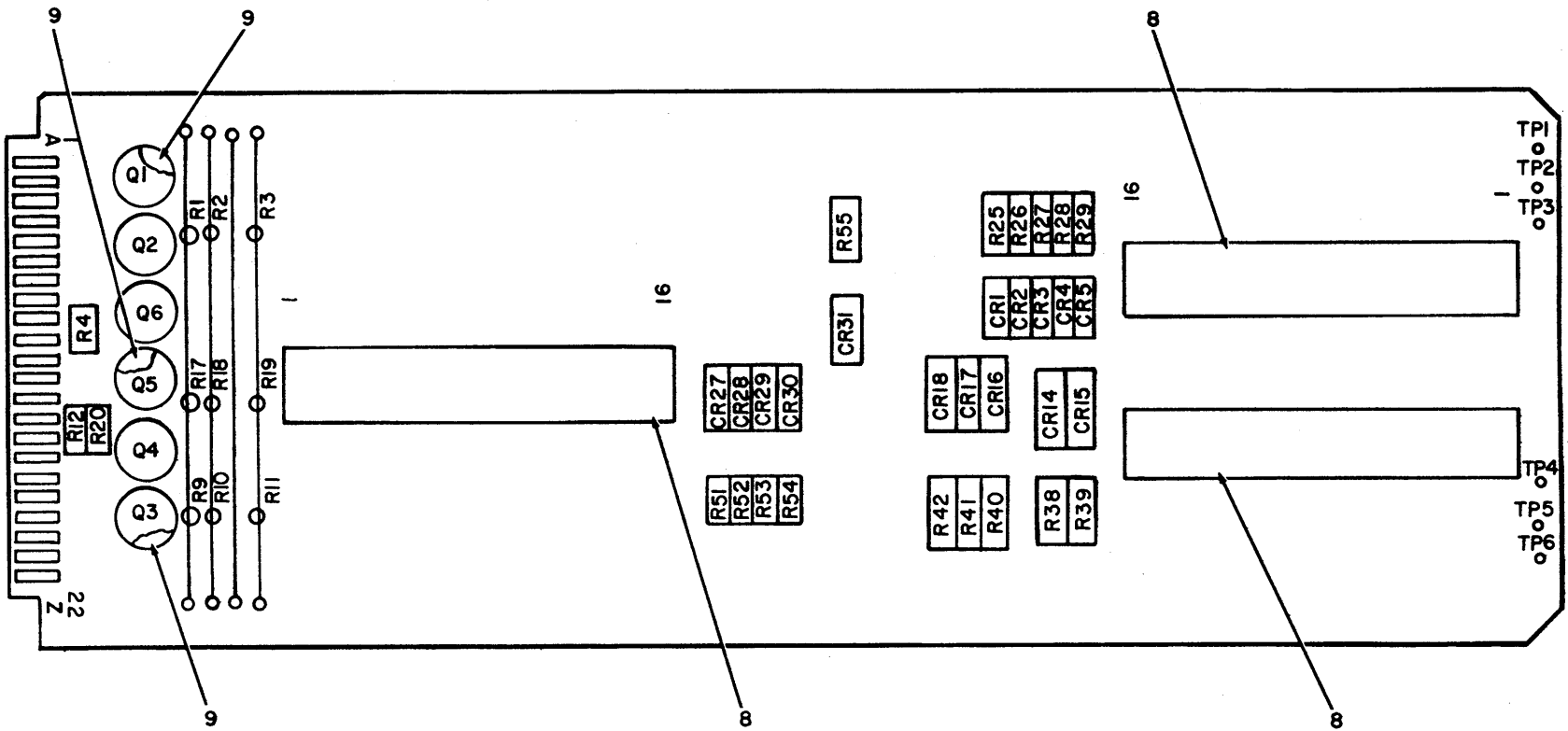
Figure 9. Component Board Assembly SMD633056 1A2A5 (Sheet 1 of 2).
