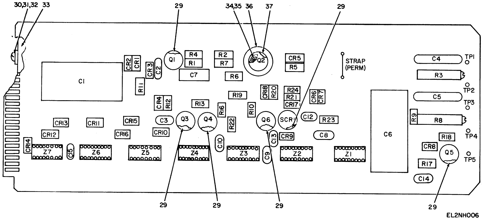
Figure 5. Component Board Assembly SMD633052 1A2A1 (Sheet 1 of 2)
