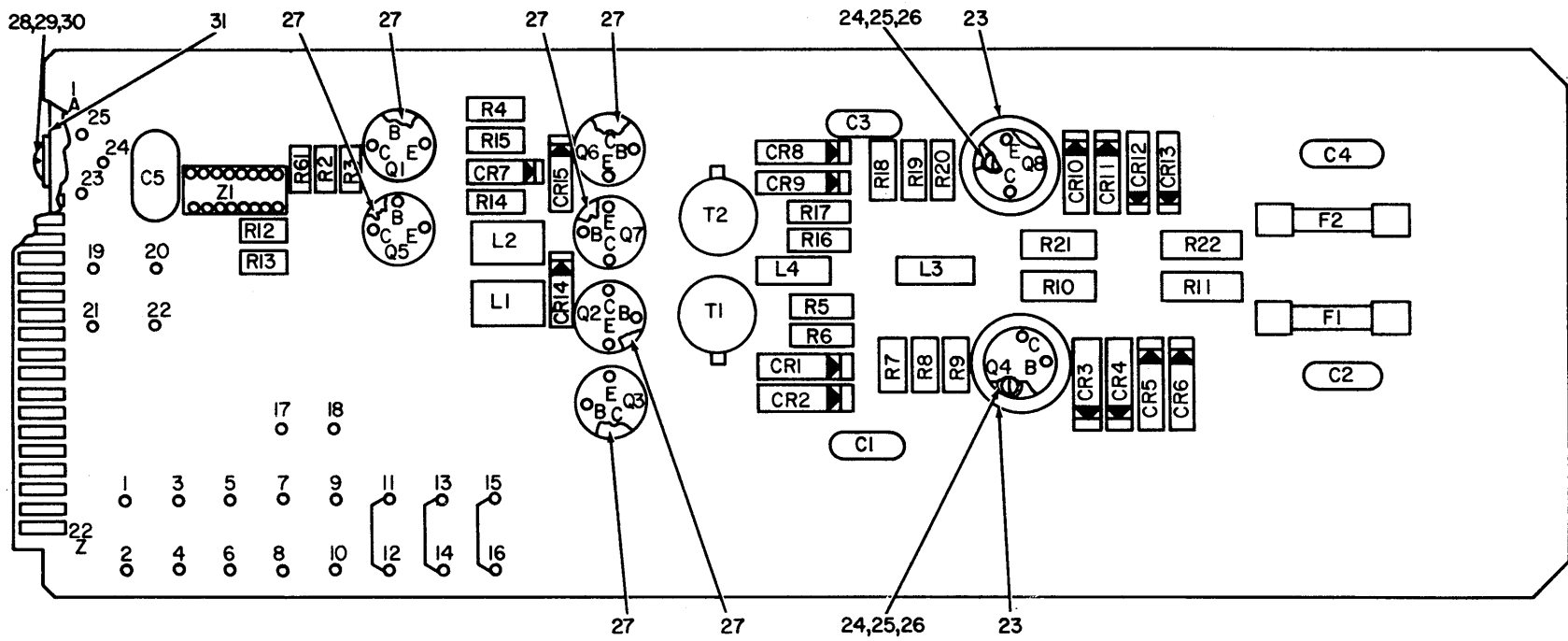
Figure 6. Component Board Assembly SMD633053 1A2A2 (Sheet 1 of 2)
