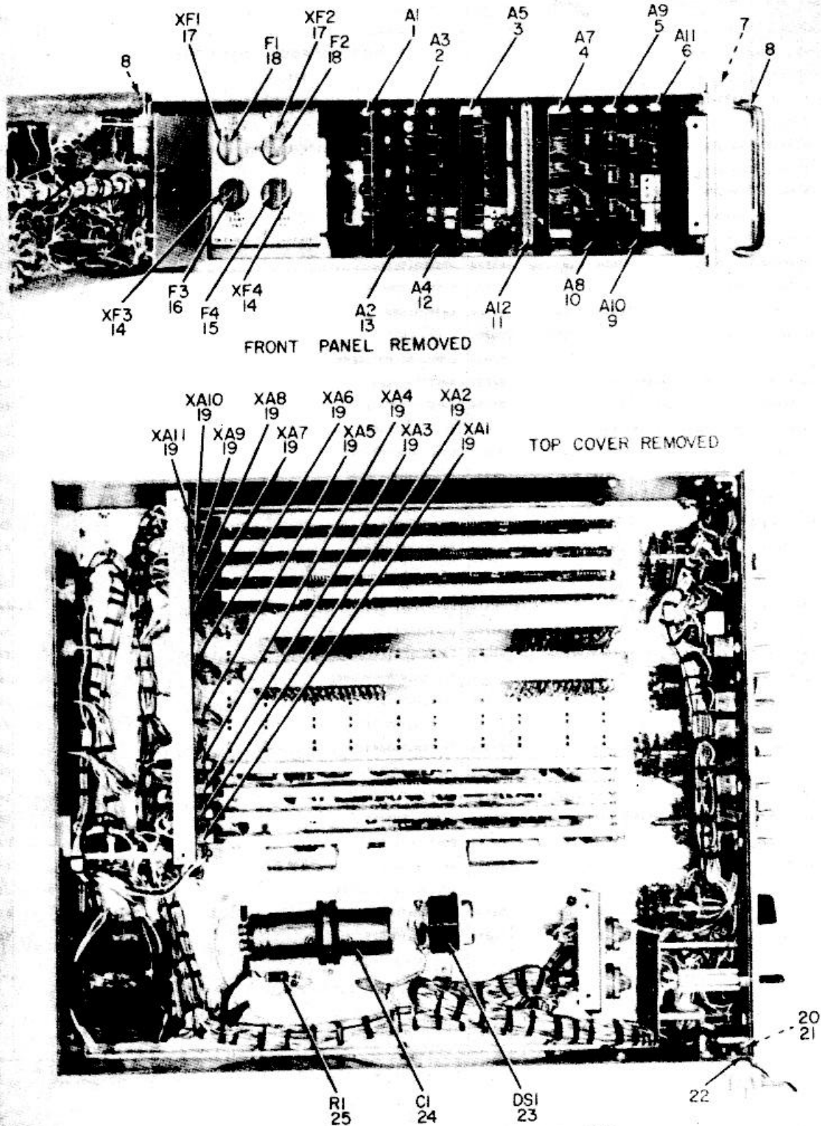
Figure 4. Chassis Assembly SMD632790 1A2.
