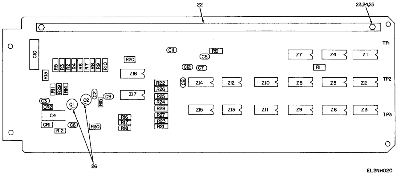
Figure 11. Component Board Assembly SMD633058 1A2A8 (Sheet 1 of 2).
