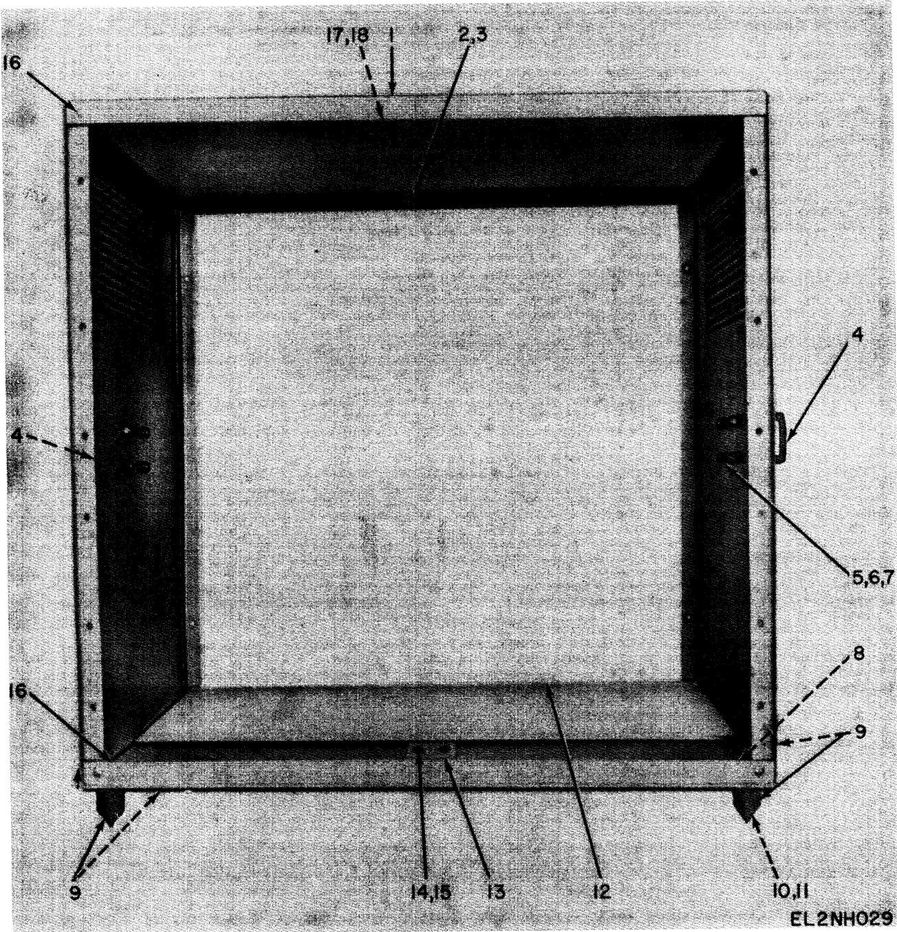
Figure 16. Case, Test Set CY-6672/GGM-15(V) (Used on V2 only).
