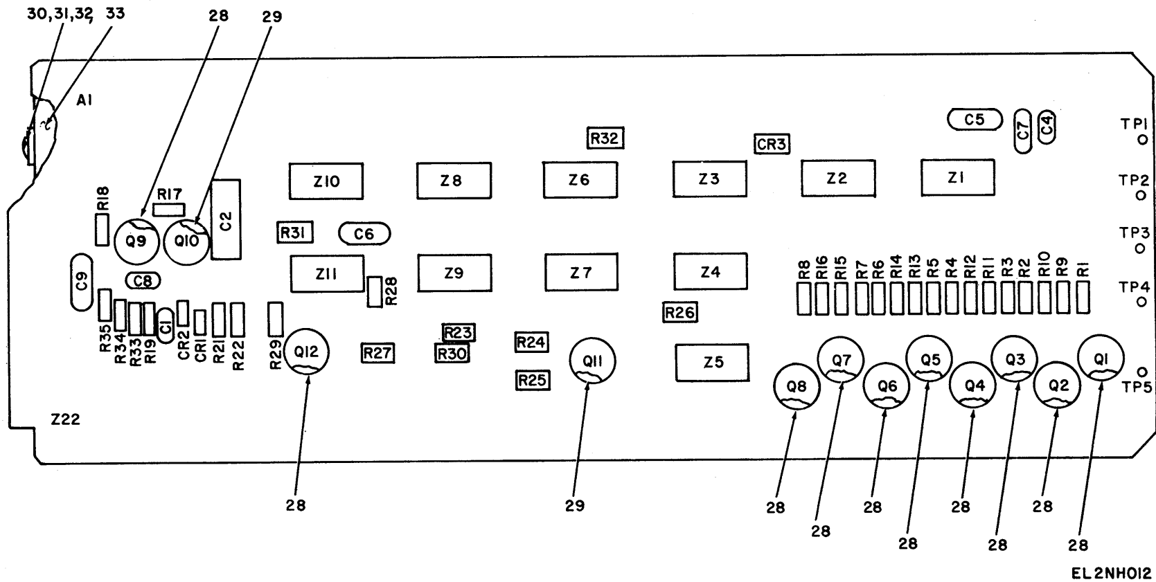
Figure 8. Component Assembly SMD633055 1A2A4 (Sheet 1 of 2).
