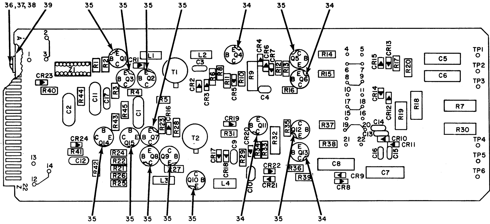
Figure 7. Component Board Assembly SMD633054 1A2A3 (Sheet 1 of 2).
