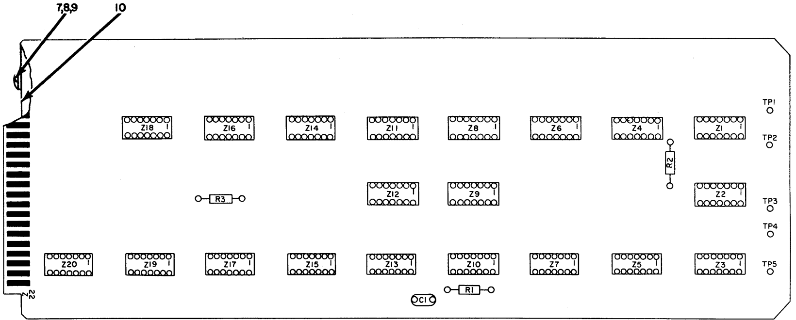
Figure 13. Component Board Assembly SMD633060 1A2A10 (Sheet 1 of 2).
