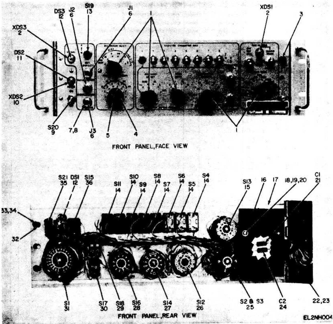
Figure 3. Panel Assembly, Front SMD632795 1A1.
