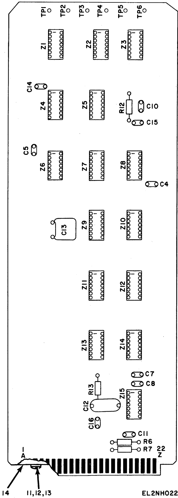
Figure 12. Component Board Assembly SMD633059 1A2A9 (Sheet 1 of 2).
